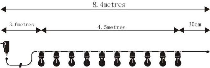
CABLE DIAGRAM
