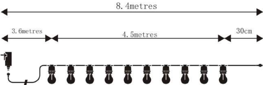
CABLE DIAGRAM
